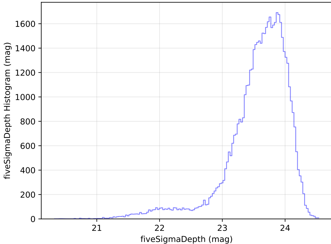
too_elab_r16_d2_giz_v3.4_10yrs Yr 1 i band: fiveSigmaDepth Histogram
