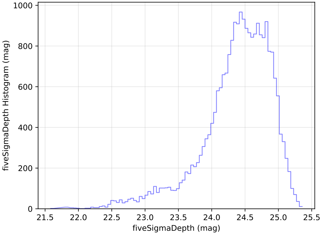
too_elab_r16_d2_giz_v3.4_10yrs Yr 1 g band: fiveSigmaDepth Histogram
