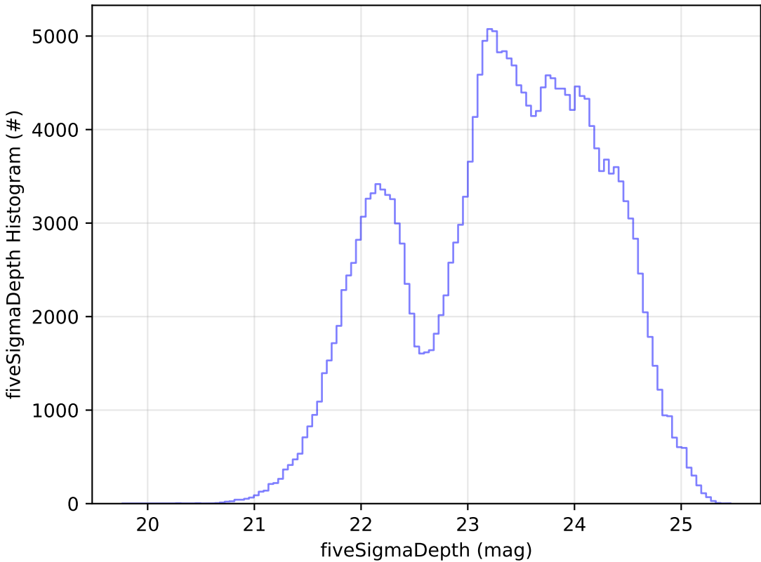
too_elab_r16_d2_giz_v3.4_10yrs Yr 1 all bands: fiveSigmaDepth Histogram
