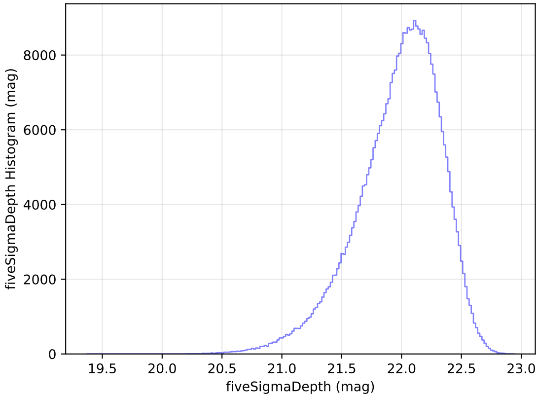
too_elab_r16_d2_giz_v3.4_10yrs WFD y band: fiveSigmaDepth Histogram
