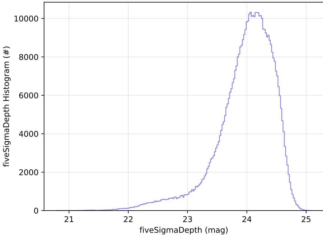
too_elab_r16_d2_giz_v3.4_10yrs WFD r band: fiveSigmaDepth Histogram
