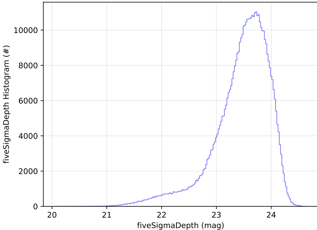
too_elab_r16_d2_giz_v3.4_10yrs WFD i band: fiveSigmaDepth Histogram
