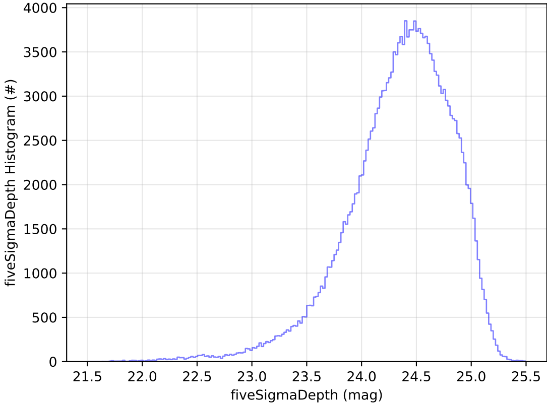
too_elab_r16_d2_giz_v3.4_10yrs WFD g band: fiveSigmaDepth Histogram
