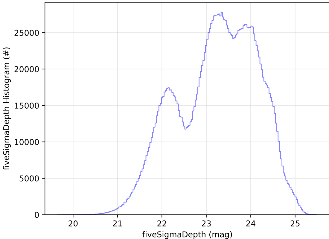
too_elab_r16_d2_giz_v3.4_10yrs WFD all bands: fiveSigmaDepth Histogram
