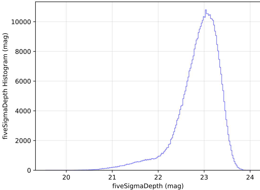
too_elab_r16_d2_giz_v3.4_10yrs All sky z band: fiveSigmaDepth Histogram
