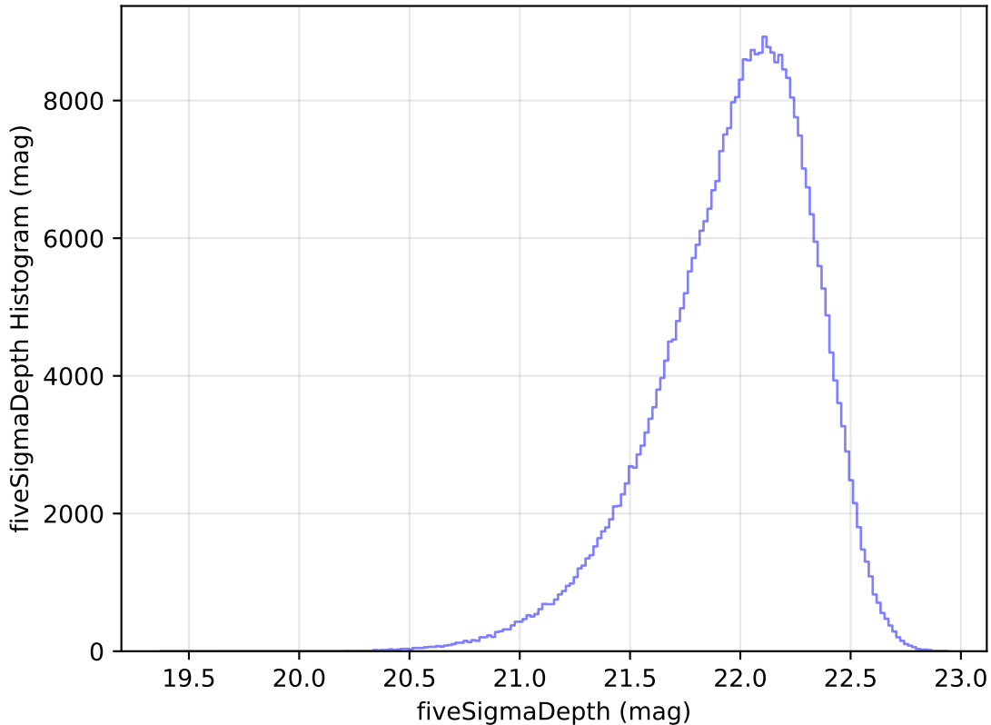
too_elab_r16_d2_giz_v3.4_10yrs All sky y band: fiveSigmaDepth Histogram
