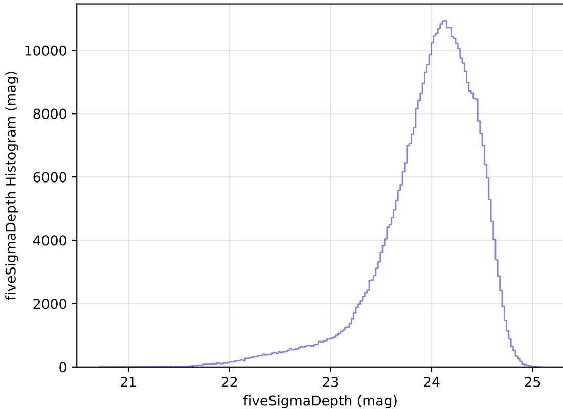
too_elab_r16_d2_giz_v3.4_10yrs All sky r band: fiveSigmaDepth Histogram
