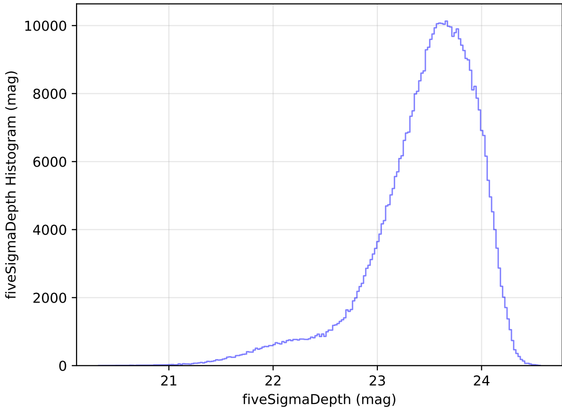
too_elab_r16_d2_giz_v3.4_10yrs All sky i band: fiveSigmaDepth Histogram
