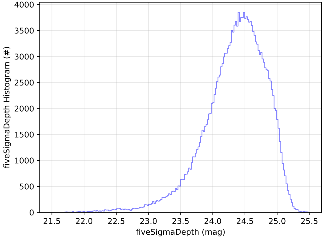
too_elab_r16_d2_giz_v3.4_10yrs All sky g band: fiveSigmaDepth Histogram
