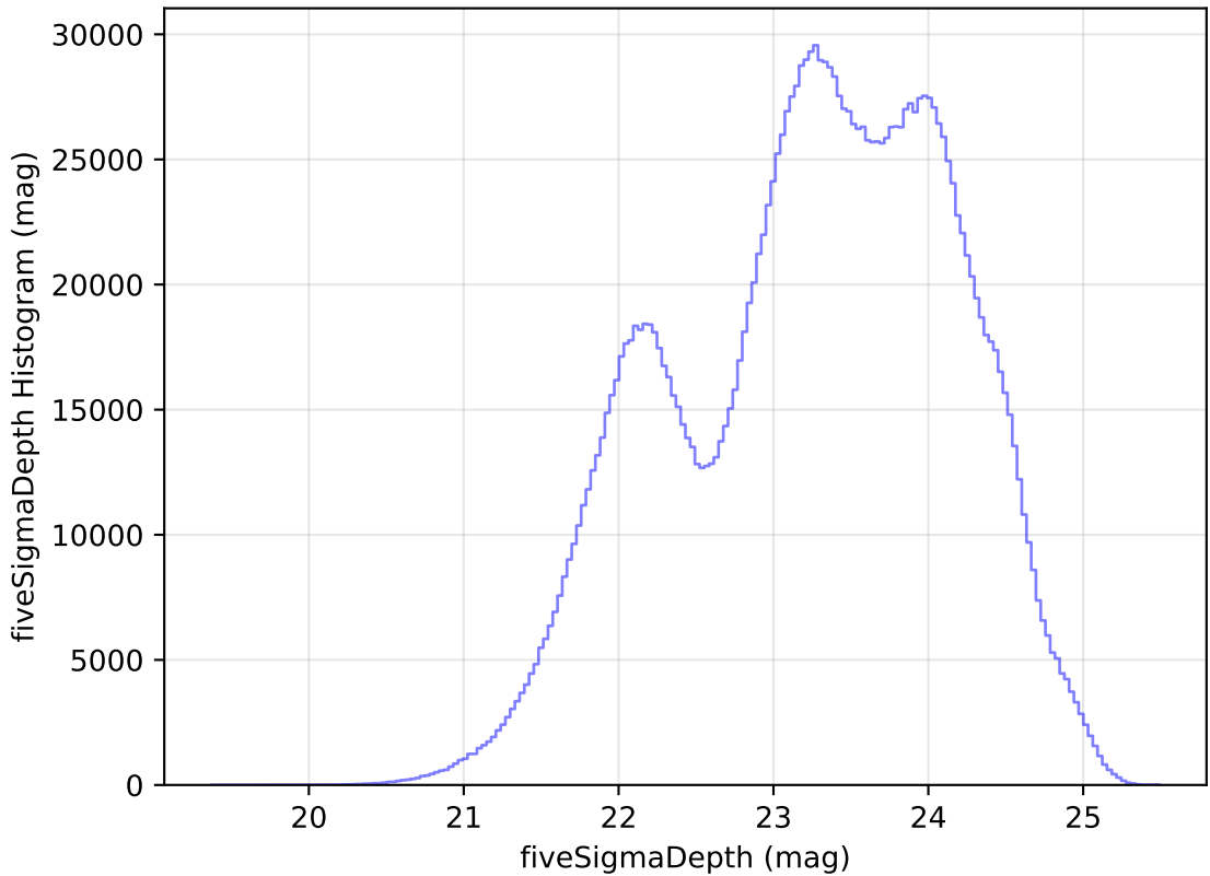
too_elab_r16_d2_giz_v3.4_10yrs All sky all bands: fiveSigmaDepth Histogram
