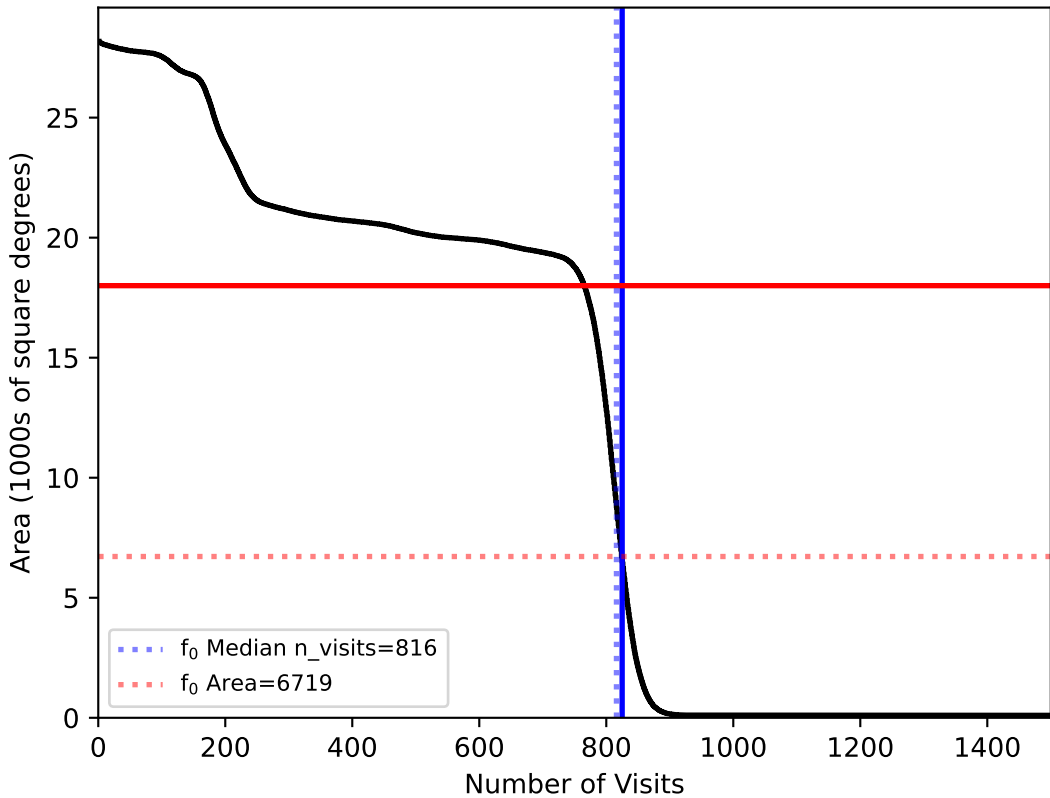
too_elab_r16_d2_giz_v3.4_10yrs All sky: f0
