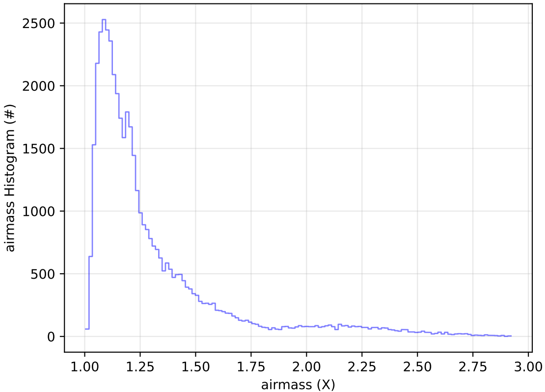
too_elab_r16_d2_giz_v3.4_10yrs Yr 1 z band: airmass Histogram
