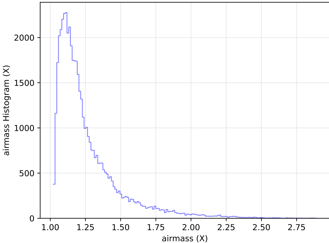
too_elab_r16_d2_giz_v3.4_10yrs Yr 1 y band: airmass Histogram
