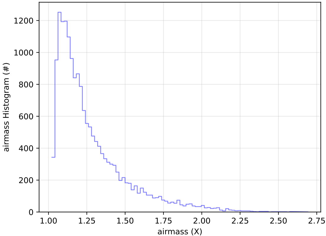
too_elab_r16_d2_giz_v3.4_10yrs Yr 1 u band: airmass Histogram
