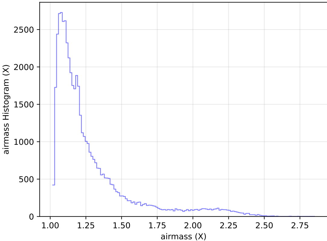
too_elab_r16_d2_giz_v3.4_10yrs Yr 1 r band: airmass Histogram
