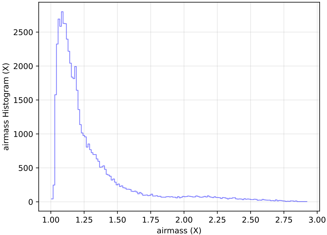
too_elab_r16_d2_giz_v3.4_10yrs Yr 1 i band: airmass Histogram
