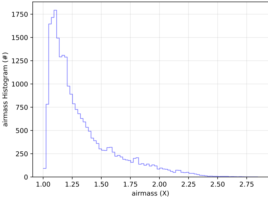
too_elab_r16_d2_giz_v3.4_10yrs Yr 1 g band: airmass Histogram
