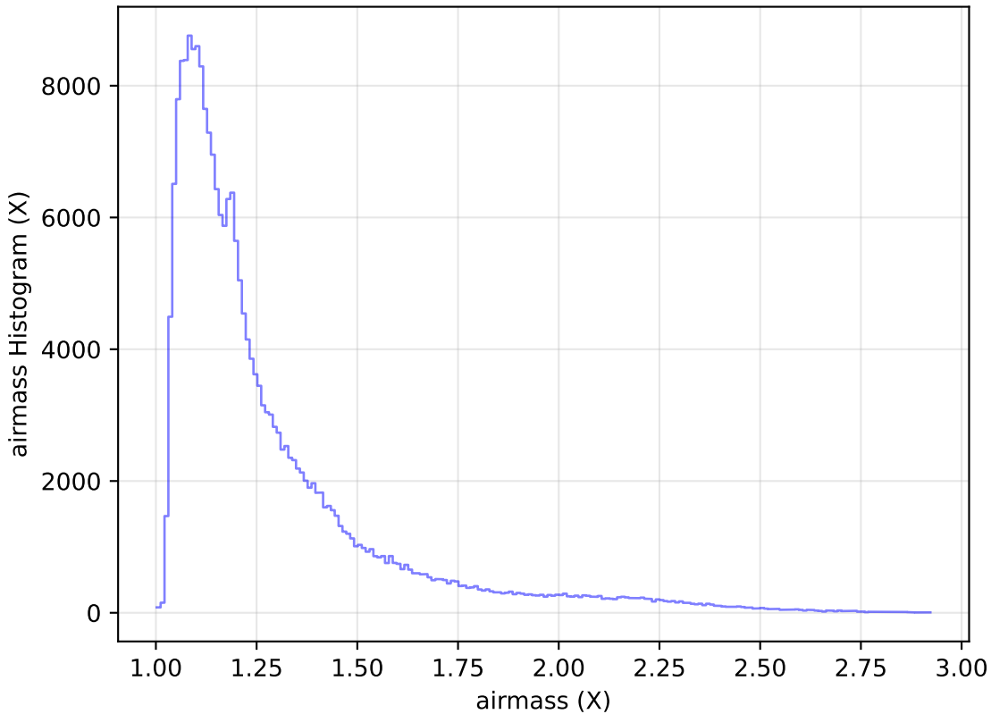
too_elab_r16_d2_giz_v3.4_10yrs Yr 1 all bands: airmass Histogram
