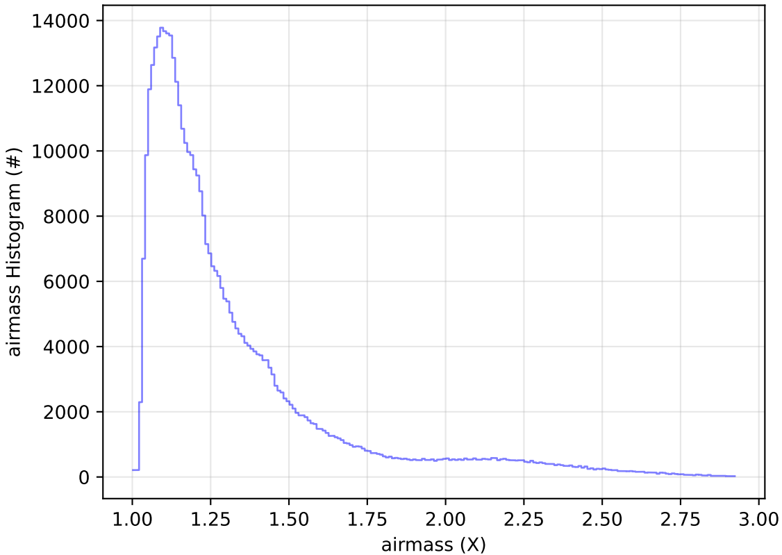
too_elab_r16_d2_giz_v3.4_10yrs WFD z band: airmass Histogram
