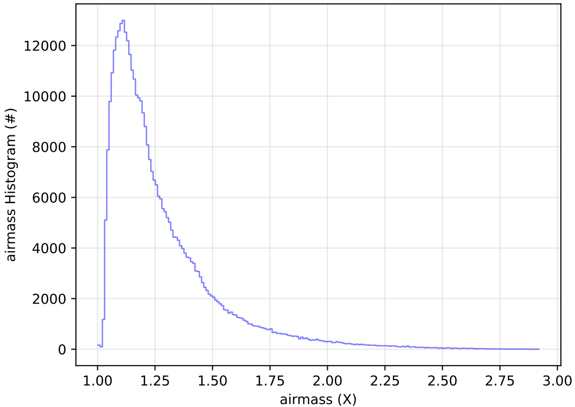
too_elab_r16_d2_giz_v3.4_10yrs WFD y band: airmass Histogram
