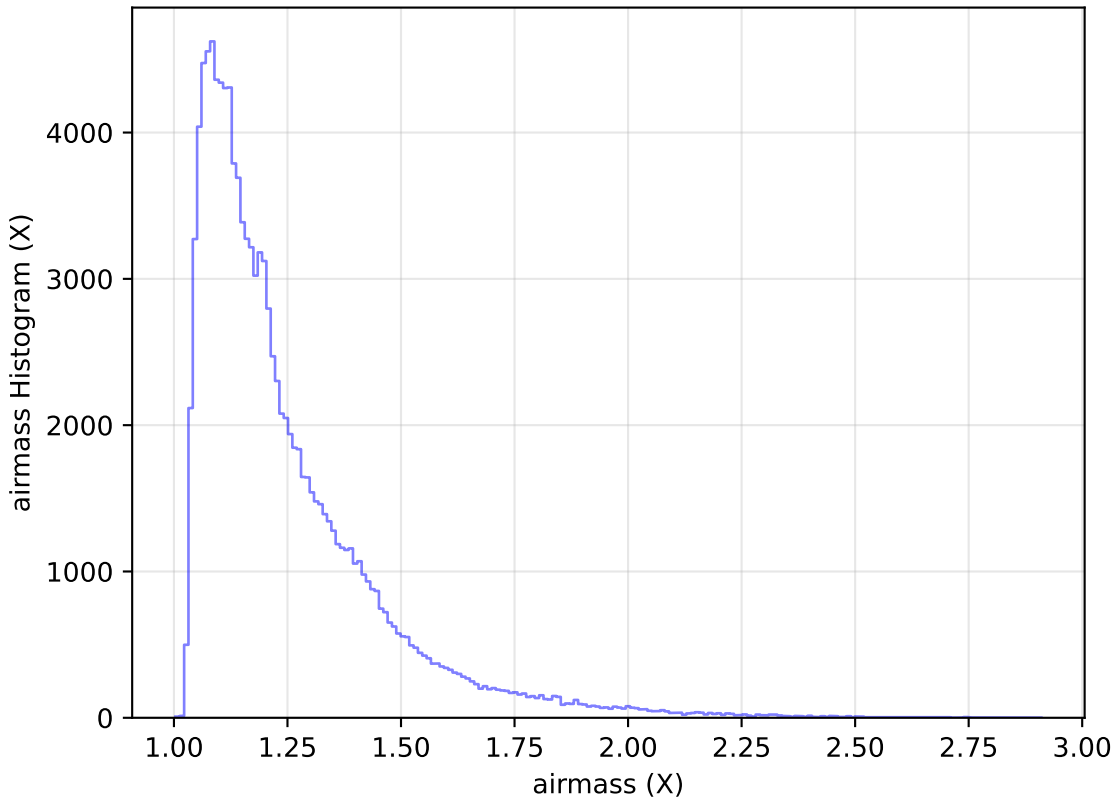
too_elab_r16_d2_giz_v3.4_10yrs WFD u band: airmass Histogram
