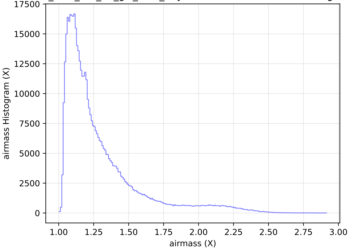
too_elab_r16_d2_giz_v3.4_10yrs WFD r band: airmass Histogram
