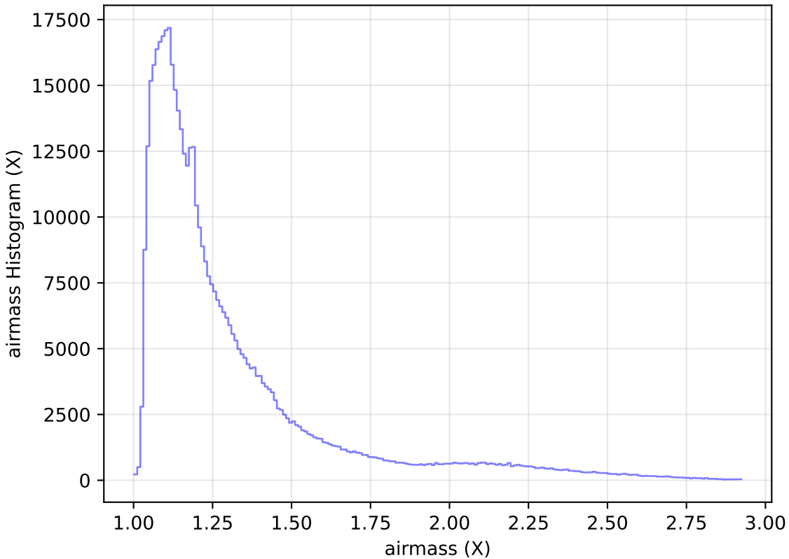
too_elab_r16_d2_giz_v3.4_10yrs WFD i band: airmass Histogram
