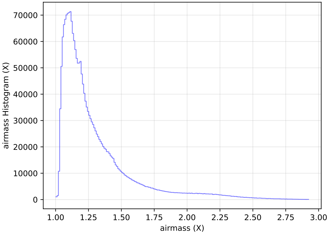
too_elab_r16_d2_giz_v3.4_10yrs WFD all bands: airmass Histogram
