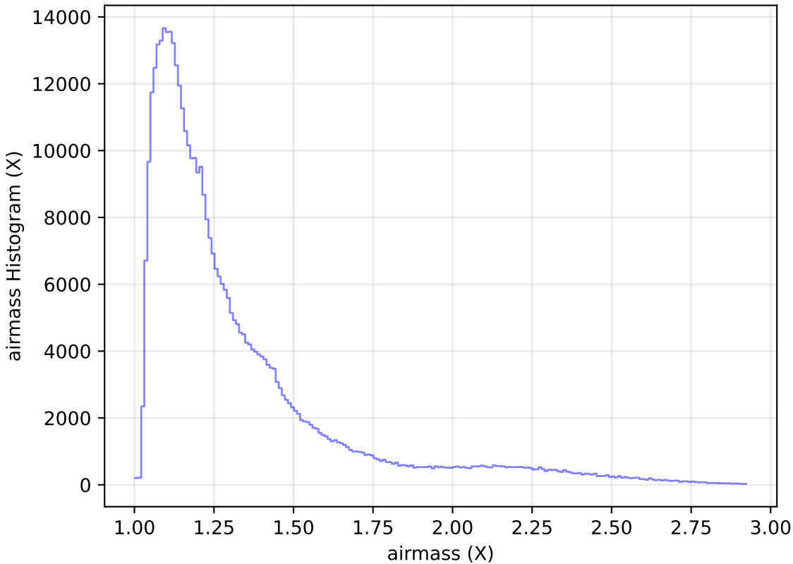
too_elab_r16_d2_giz_v3.4_10yrs All sky z band: airmass Histogram
