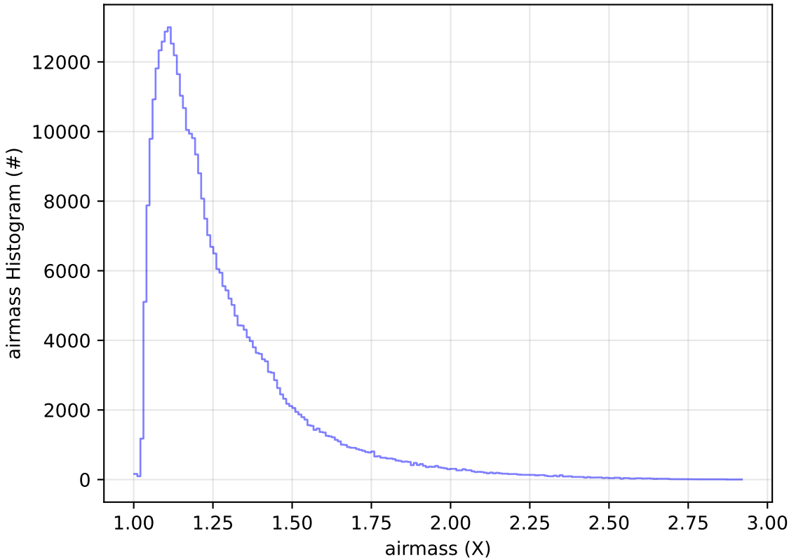
too_elab_r16_d2_giz_v3.4_10yrs All sky y band: airmass Histogram
