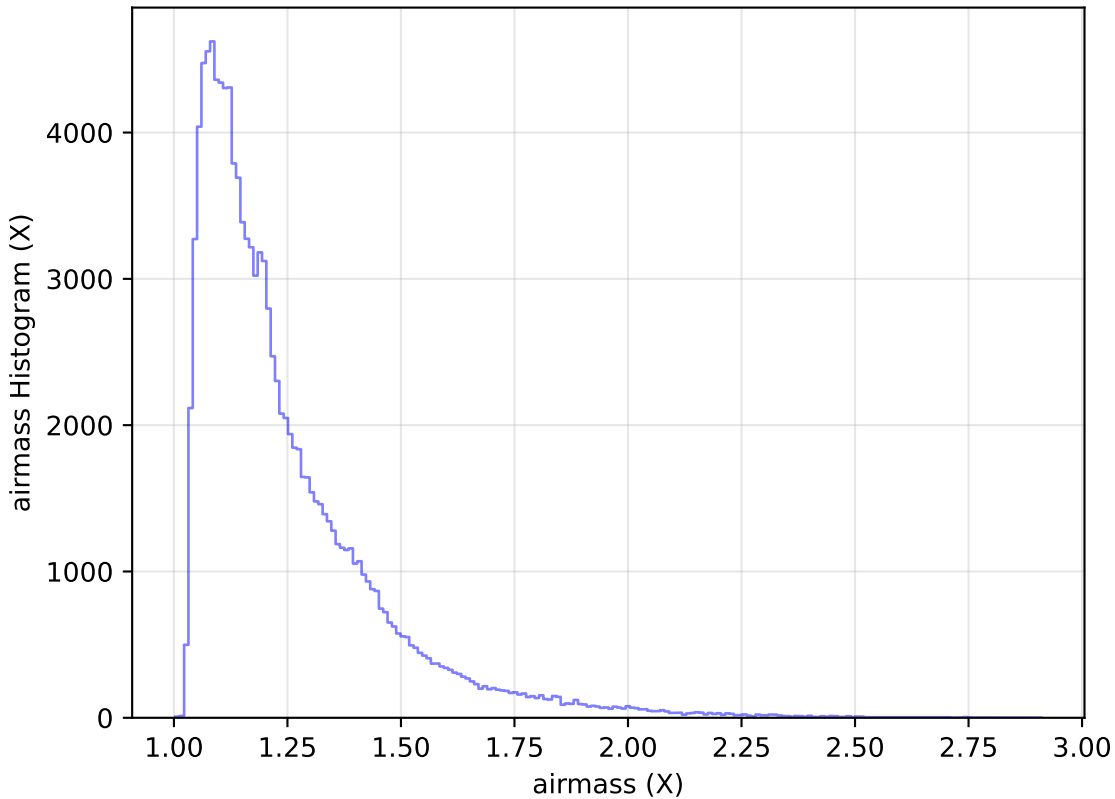
too_elab_r16_d2_giz_v3.4_10yrs All sky u band: airmass Histogram
