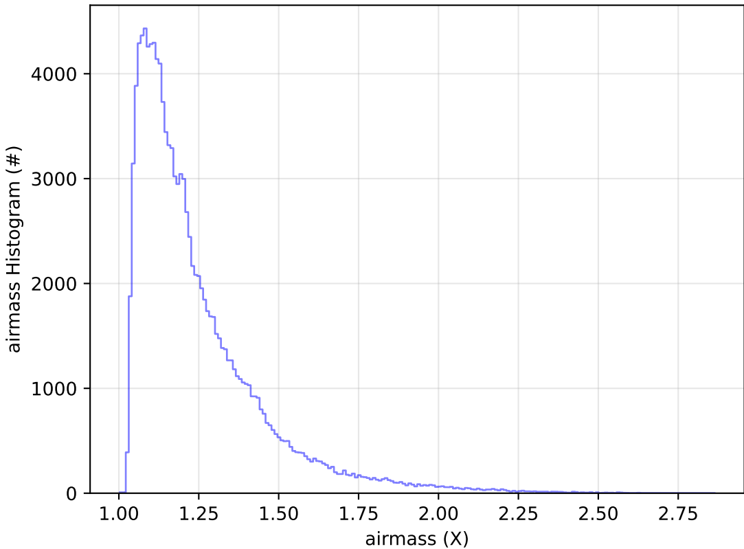
too_elab_r16_d2_giz_v3.4_10yrs All sky u band: airmass Histogram
