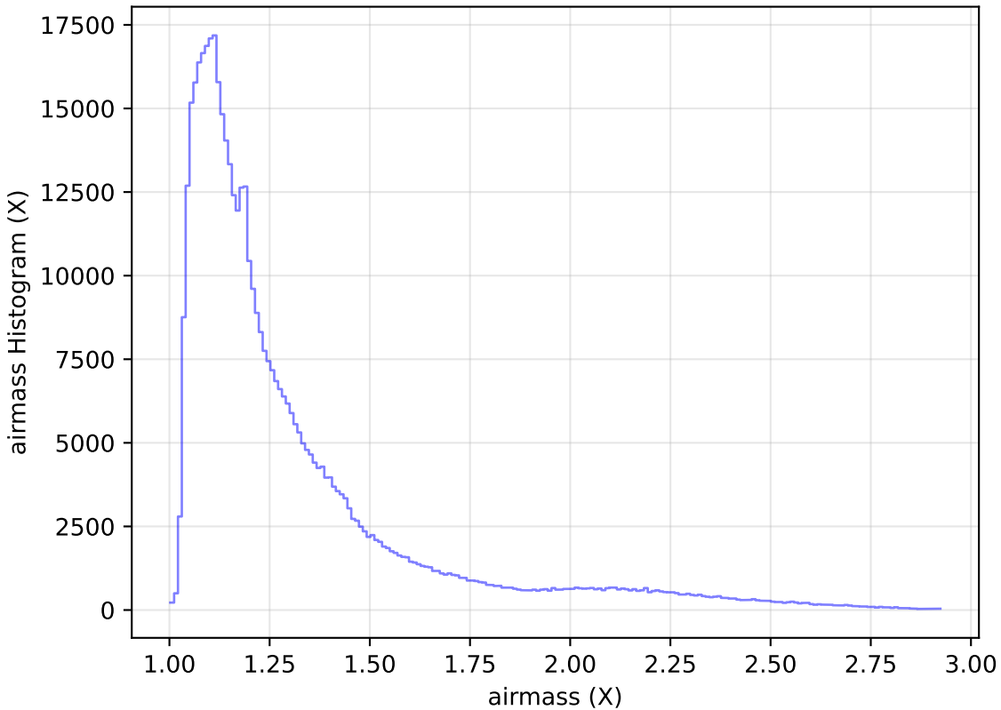
too_elab_r16_d2_giz_v3.4_10yrs All sky i band: airmass Histogram
