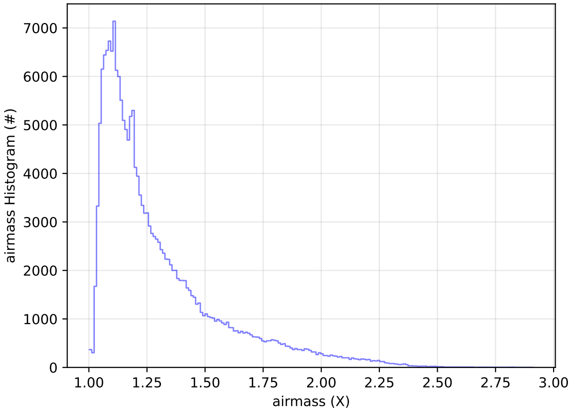
too_elab_r16_d2_giz_v3.4_10yrs All sky g band: airmass Histogram
