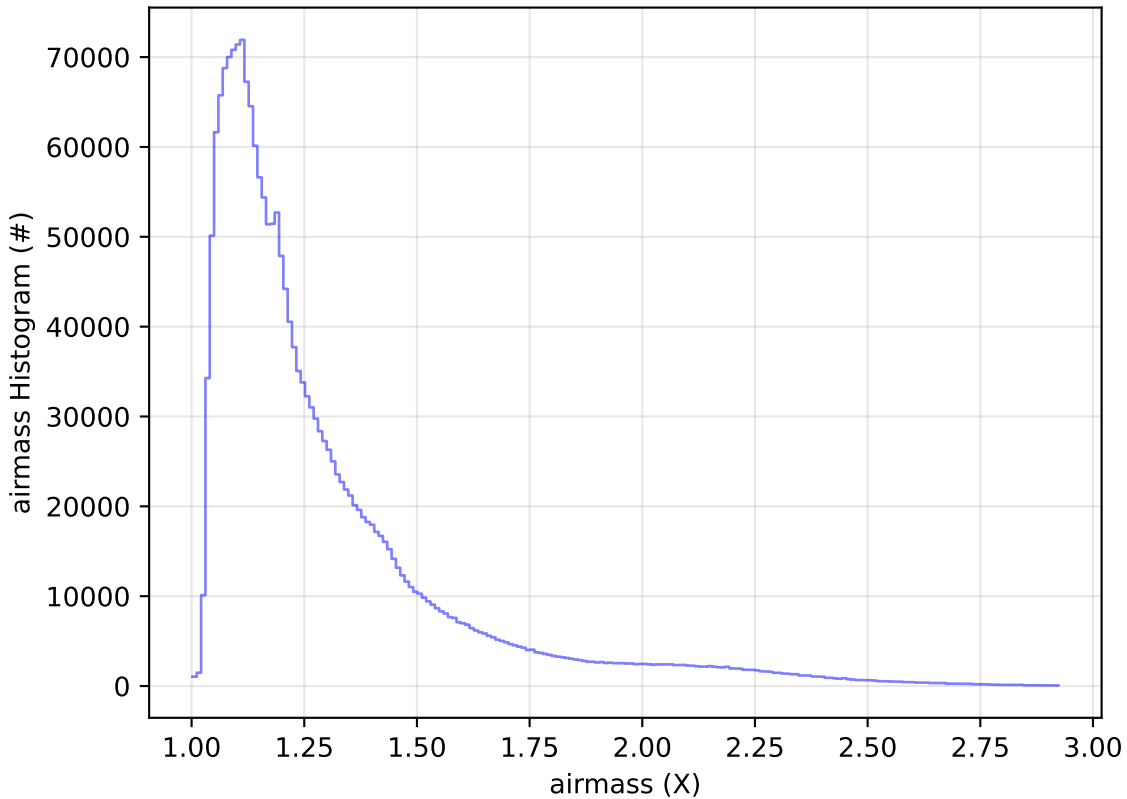
too_elab_r16_d2_giz_v3.4_10yrs All sky all bands: airmass Histogram
