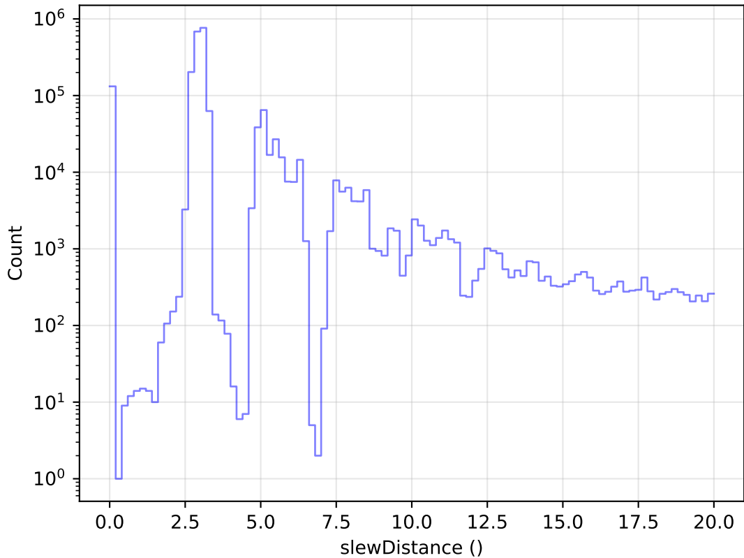
too_elab_r16_d2_giz_v3.4_10yrs All visits: Zoom Slew Distance Histogram
