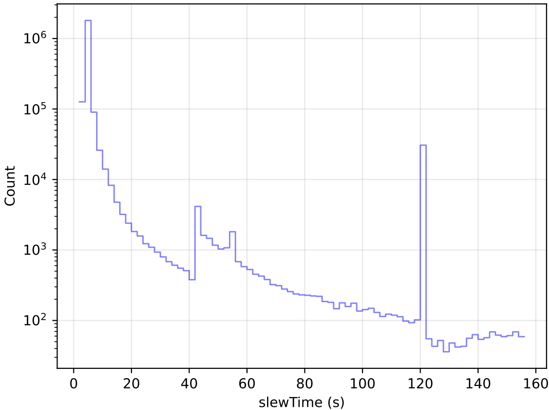
too_elab_r16_d2_giz_v3.4_10yrs All visits: Slew Time Histogram
