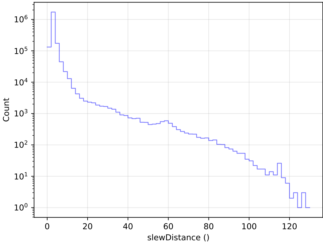
too_elab_r16_d2_giz_v3.4_10yrs All visits: Slew Distance Histogram
