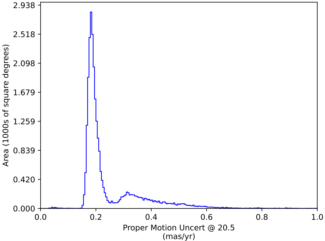
too_elab_r16_d2_giz_v3.4_10yrs All sky: Proper Motion Uncert @ 20.5
