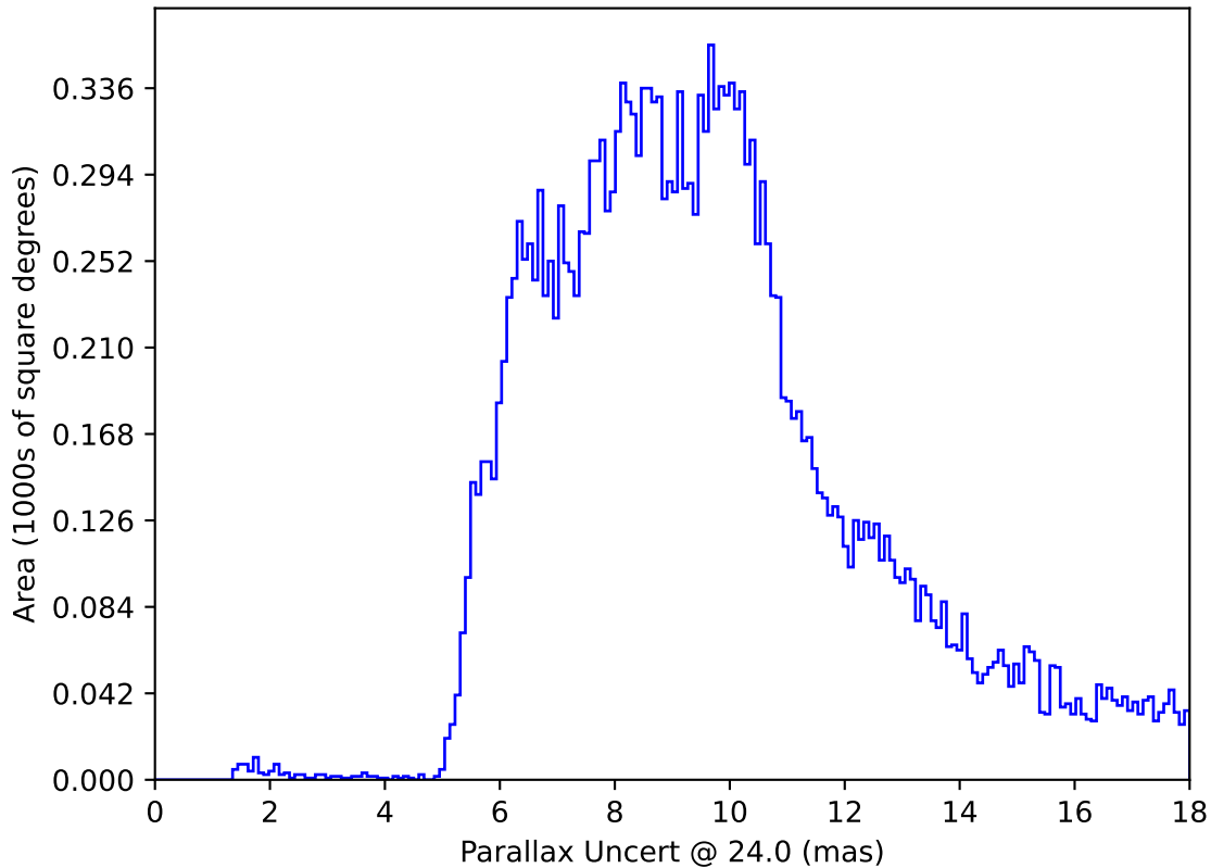
too_elab_r16_d2_giz_v3.4_10yrs All sky: Parallax Uncert @ 24.0
