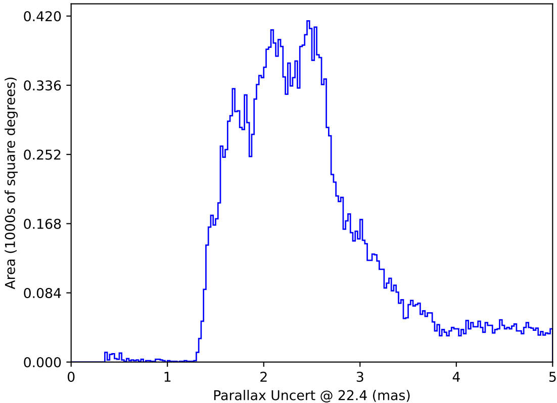
too_elab_r16_d2_giz_v3.4_10yrs All sky: Parallax Uncert @ 22.4
