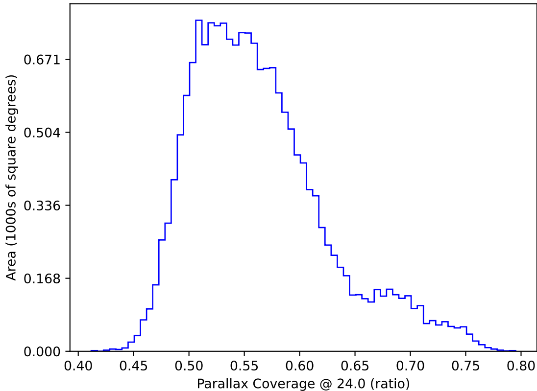
too_elab_r16_d2_giz_v3.4_10yrs WFD: Parallax Coverage @ 24.0
