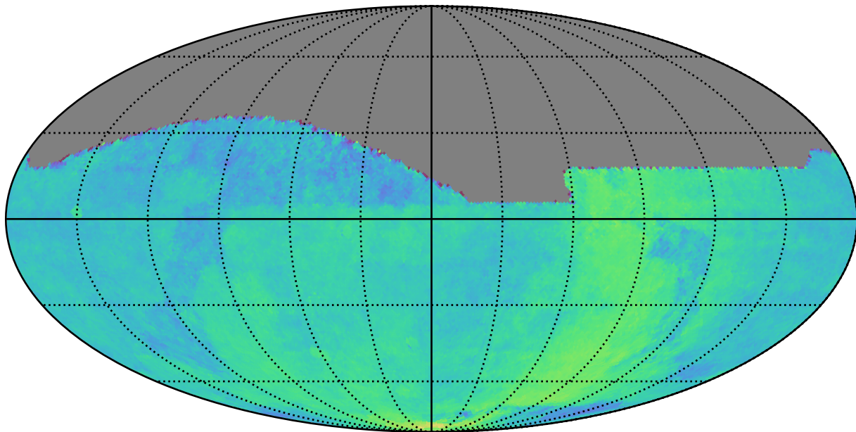
too_elab_r16_d2_giz_v3.4_10yrs All sky: Parallax Coverage @ 24.0
