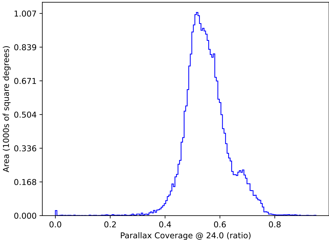
too_elab_r16_d2_giz_v3.4_10yrs All sky: Parallax Coverage @ 24.0
