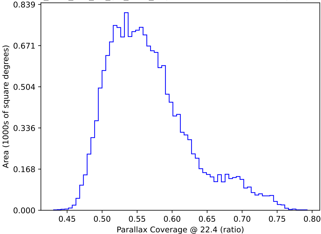
too_elab_r16_d2_giz_v3.4_10yrs WFD: Parallax Coverage @ 22.4
