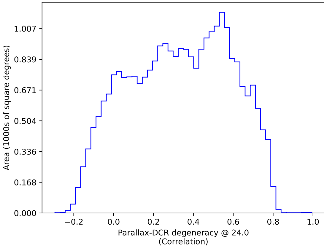
too_elab_r16_d2_giz_v3.4_10yrs All sky: Parallax-DCR degeneracy @ 24.0
