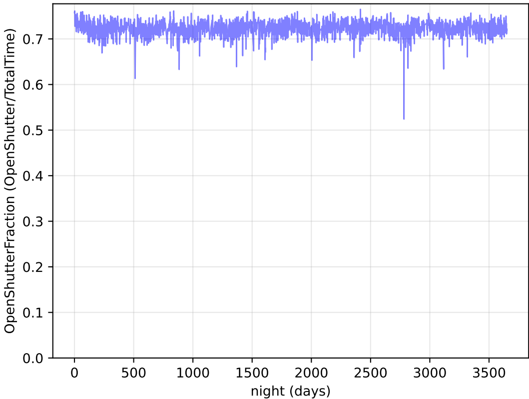
too_elab_r16_d2_giz_v3.4_10yrs Per night: OpenShutterFraction
