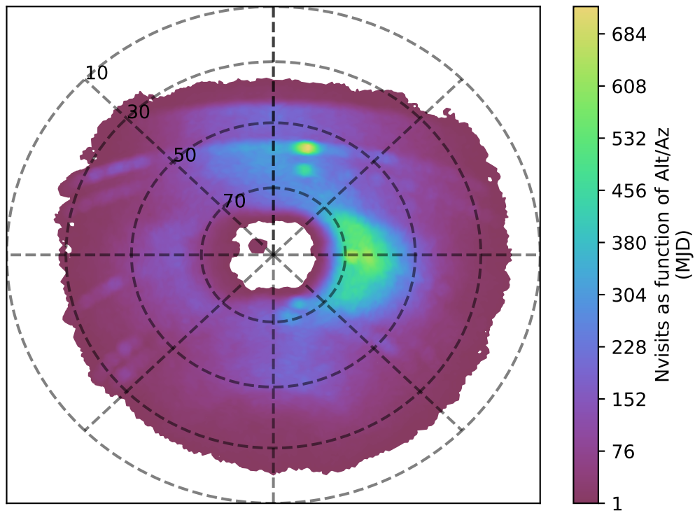
too_elab_r16_d2_giz_v3.4_10yrs u band: Nvisits as function of Alt/Az
