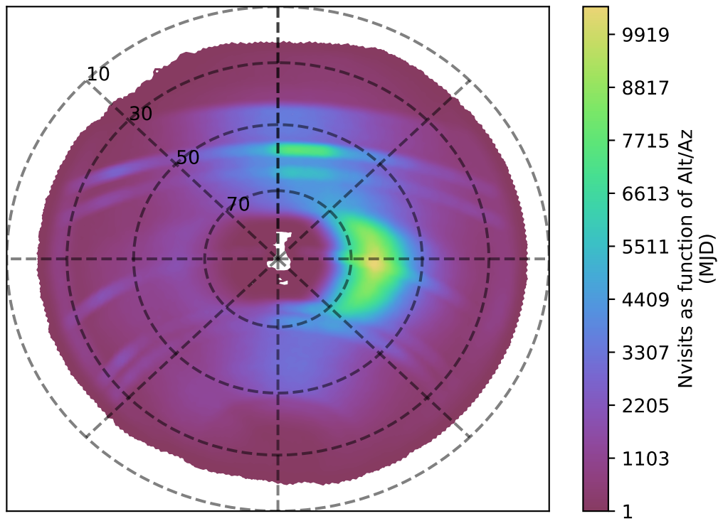
too_elab_r16_d2_giz_v3.4_10yrs all bands: Nvisits as function of Alt/Az
