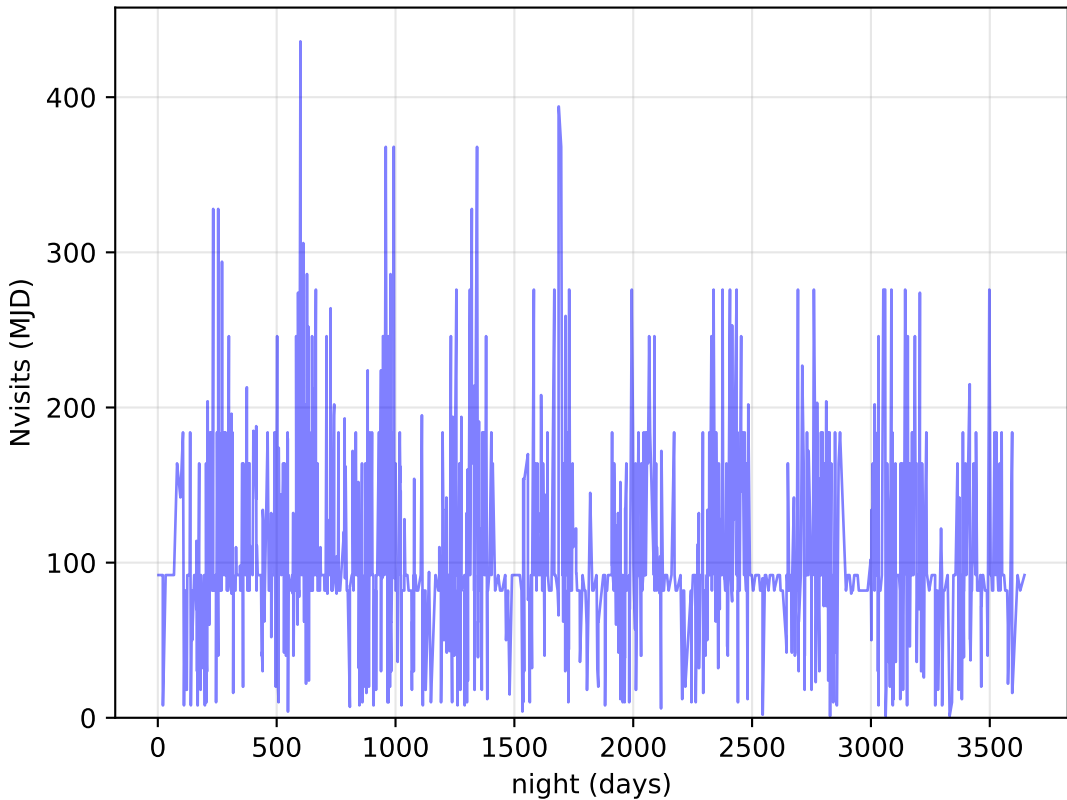
too_elab_r16_d2_giz_v3.4_10yrs DDF: Nvisits
