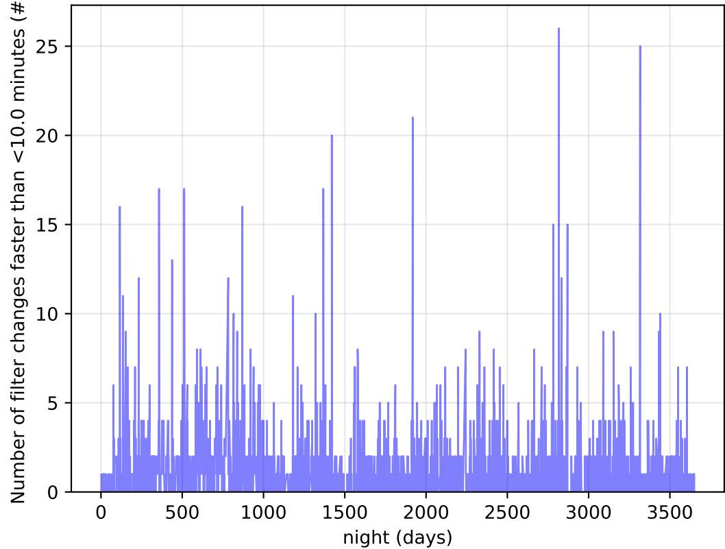
too_elab_r16_d2_giz_v3.4_10yrs Per Night: Number of filter changes faster than <10.0 minutes
